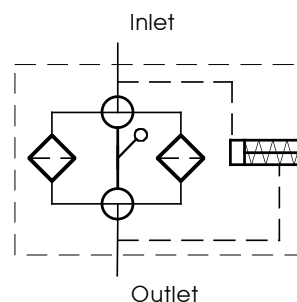
Circuit Symbol
